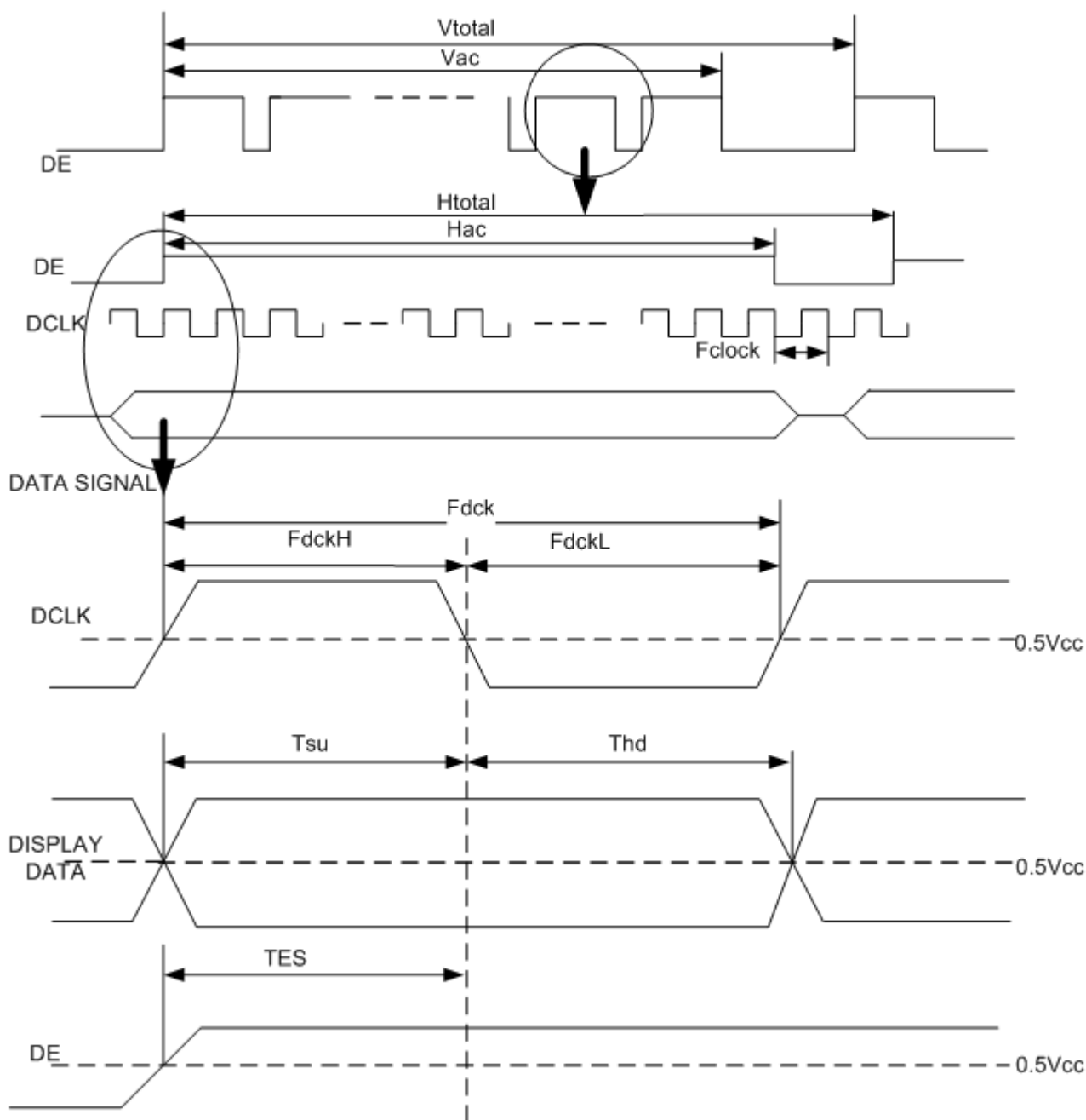
Figure 13 Timing Characteristics
