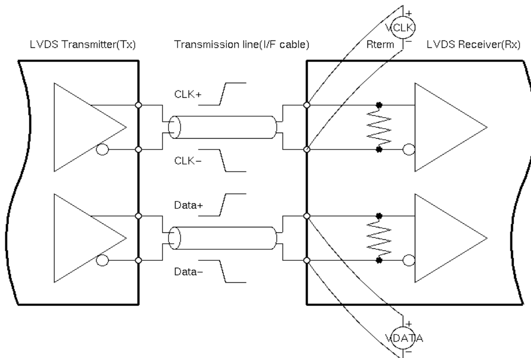
Figure 10 Measurement System
