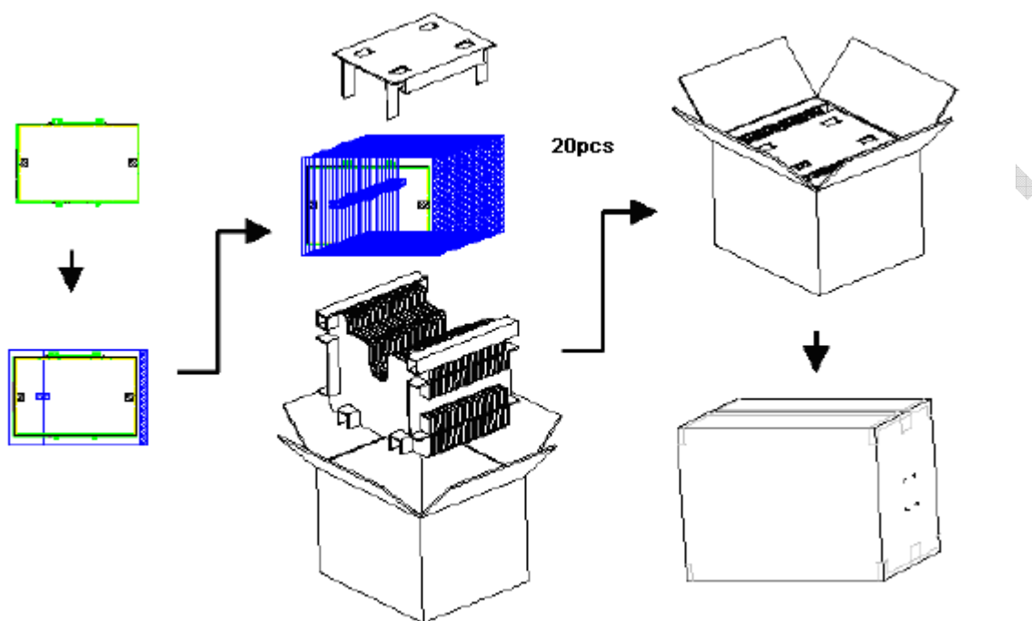
Figure 20 Packing Method
